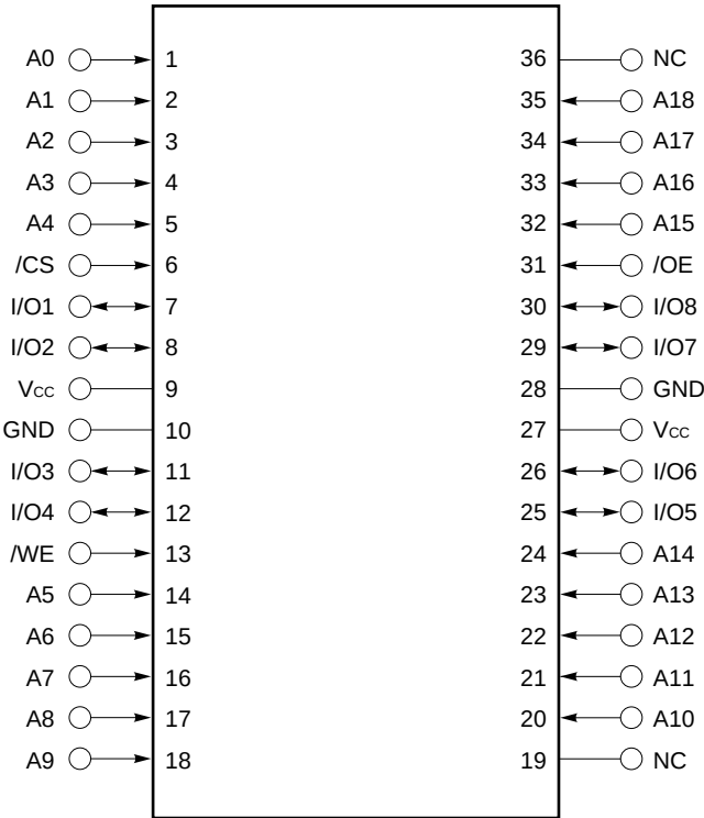
36-pin PLASTIC SOJ (10.16 mm (400))
