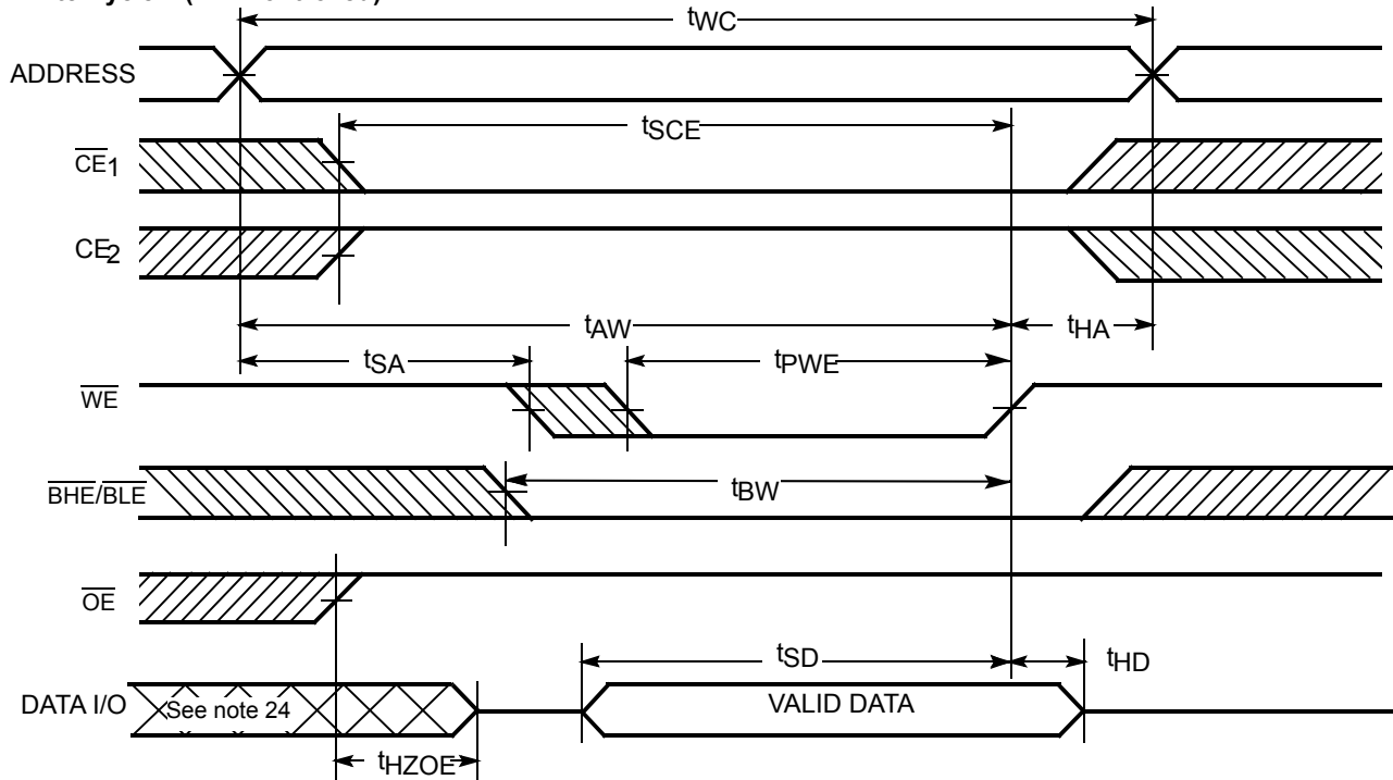
Write Cycle 2 ( \overline{CE_1} or CE_2 Controlled) [19, 23, 24, 25]
