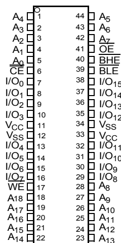
44 TSOP II Top View
