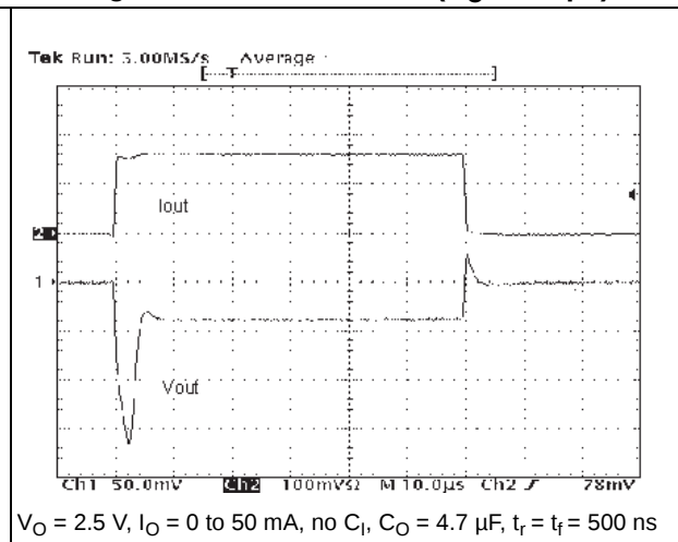
Figure 16. Load transient ( C_O = 4.7 \mu F)
