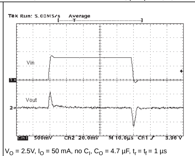
Figure 14. Line transient ( t_r = t_f = 1 \mu s)
