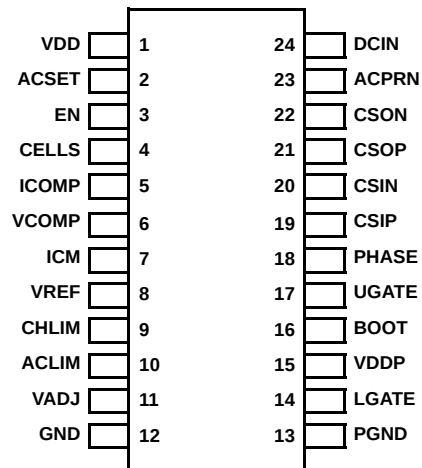
ISL6252, ISL6252A (24 LD QSOP) TOP VIEW
