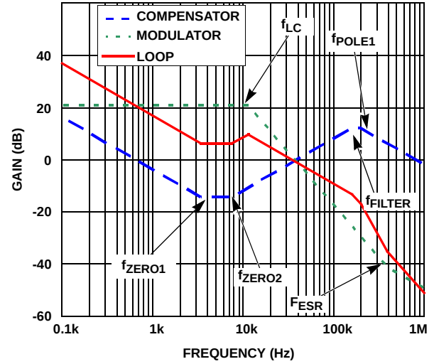
FIGURE 24. ASYMPTOTIC BODE PLOT OF THE VOLTAGE CONTROL LOOP GAIN
