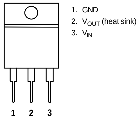
TO-220 Top View
