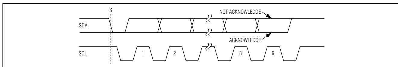
Figure 8. Acknowledge Bits
