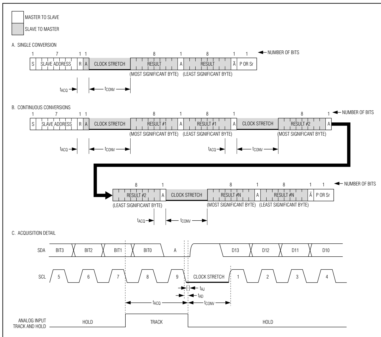
Figure 11. Read Cycle
