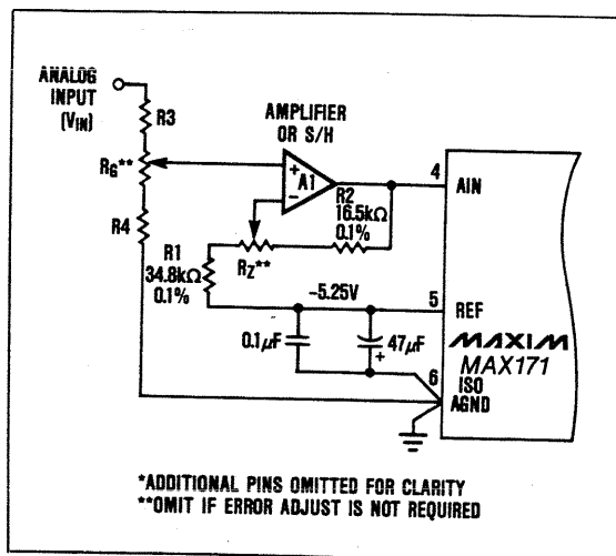
Figure 8. MAX171 Non-Inverting Bipolar Operation
