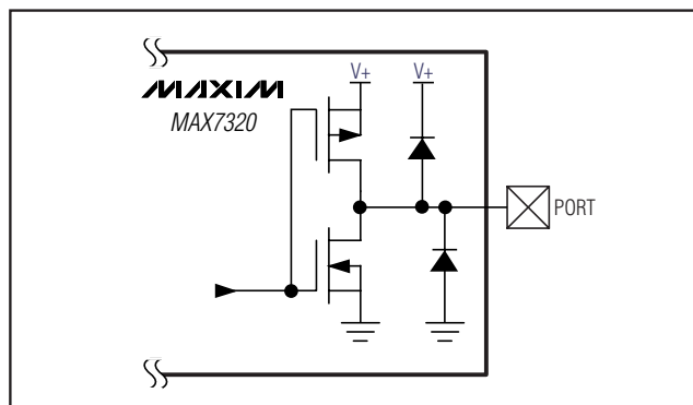
Figure 8. Output Port Structure
