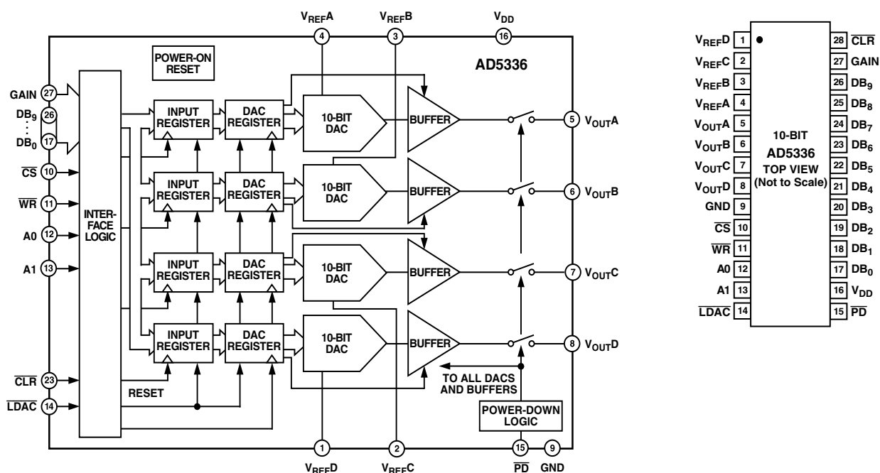
AD5336 PIN CONFIGURATION
