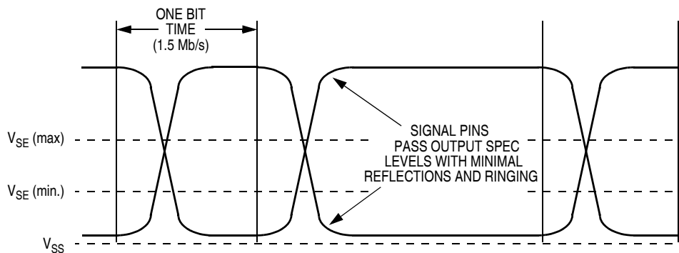
Figure 11-11. Receiver Characteristics
