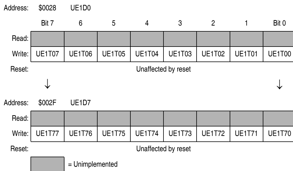
Figure 11-27. USB Endpoint 1 Data Registers (UE1D0–UE1D7)
