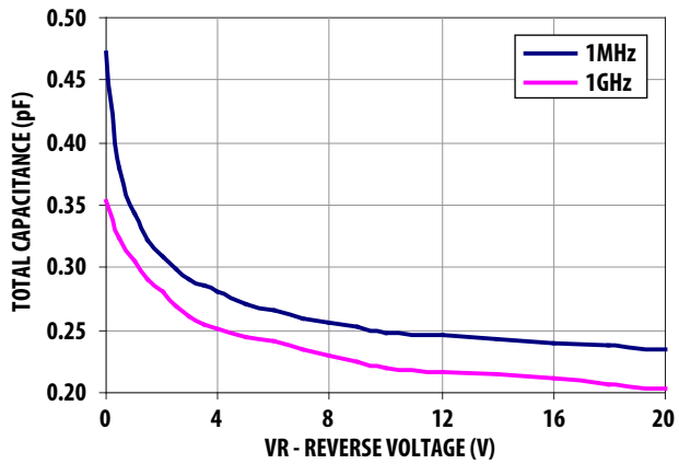
Figure 3. Total Capacitance vs. Reverse Voltage
