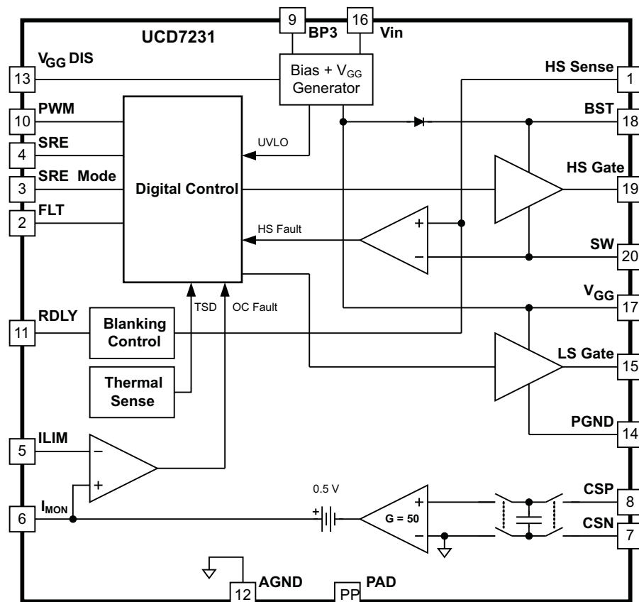
Figure 1. UCD7231 Block Diagram
