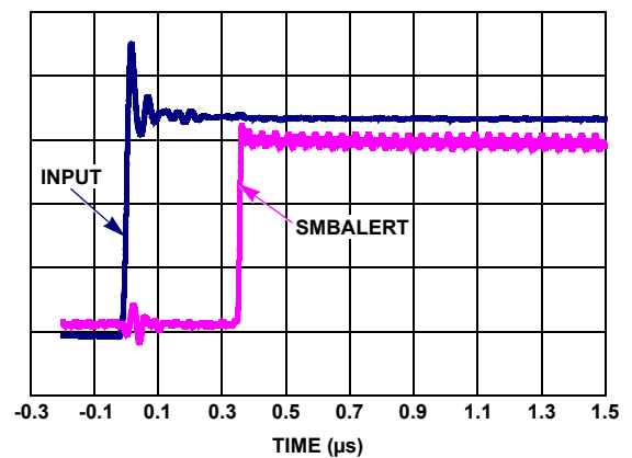
FIGURE 86. 0V or UV or OC ALERT RESPONSE TIME
