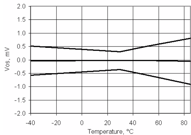
Figure 11-3. Opamp Voffset vs Temperature, V_{dda} = 5\text{ V}
