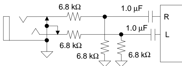
Figure 26. Line Inputs
