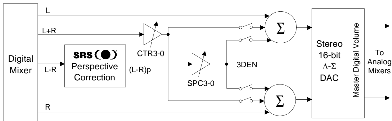
Figure 7. SRS Block Diagram
