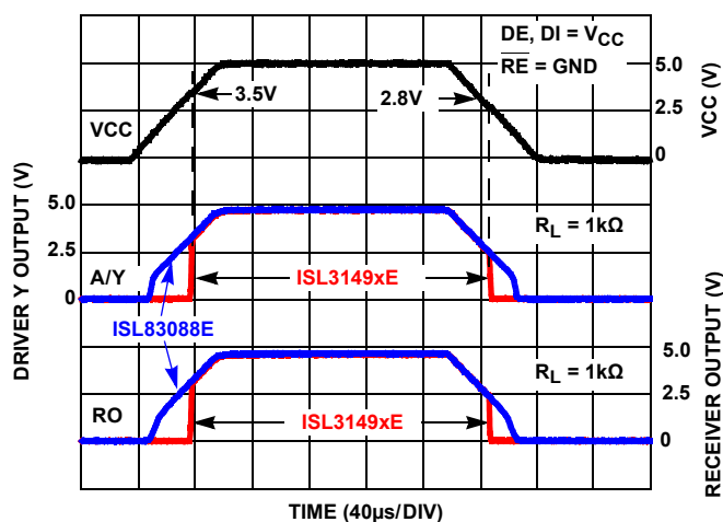
FIGURE 9. HOT PLUG PERFORMANCE (ISL3149xE) vs ISL83088E WITHOUT HOT PLUG CIRCUITRY
