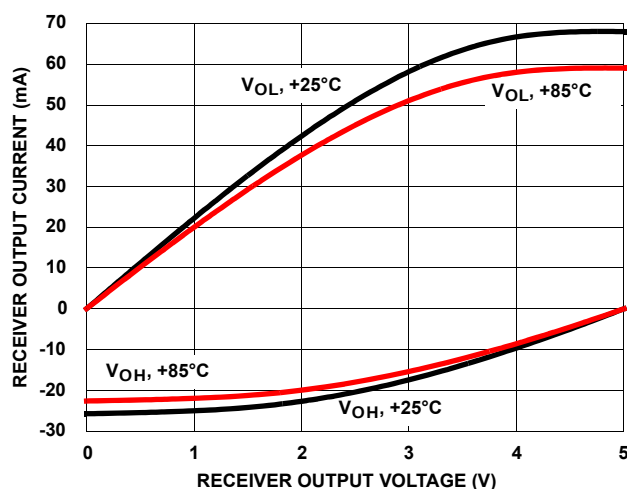
FIGURE 13. RECEIVER OUTPUT CURRENT vs RECEIVER OUTPUT VOLTAGE
