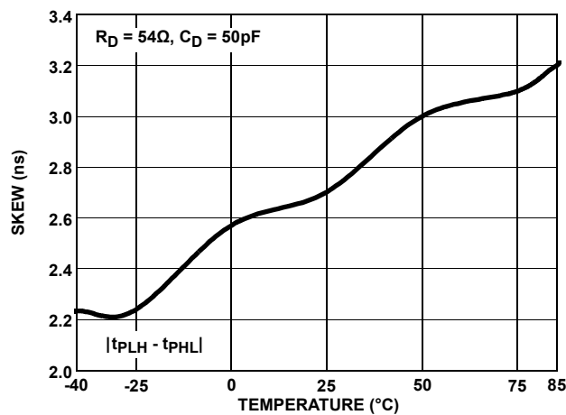
FIGURE 20. DRIVER DIFFERENTIAL SKEW vs TEMPERATURE (ISL31496E, ISL31498E)
