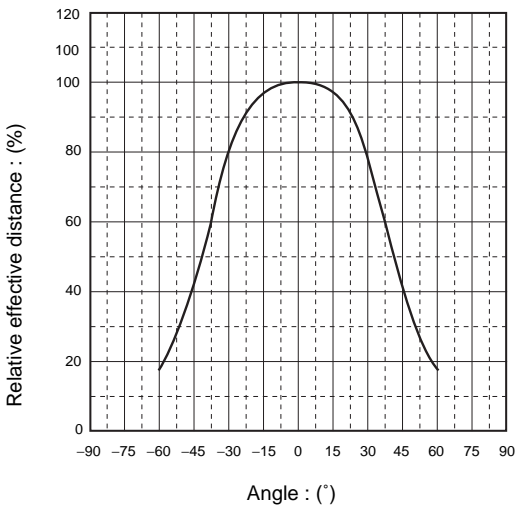
Fig.7 Direction characteristic (Horizontal direction)
