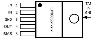
Figure 2. TO-220 – Top View See Package Number NDH0005D
