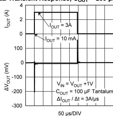
Load Transient Response, C_{OUT} = 100\text{ }\mu\text{F} Tantalum
