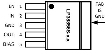
Figure 1. DDPAK/TO-263 – Top View See Package Number KTT0005B
