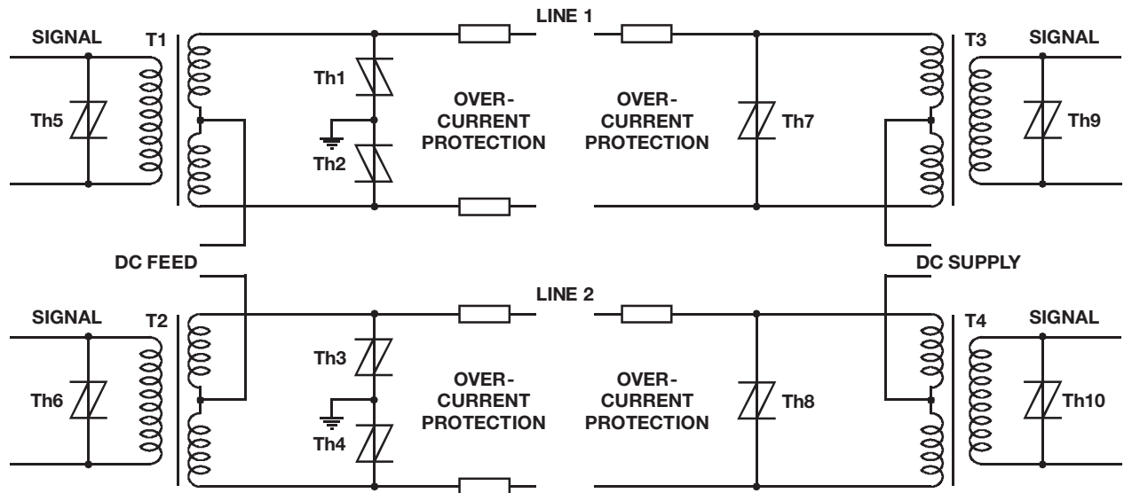
TRANSFORMER COUPLED FOUR-WIRE INTERFACE
