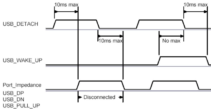
Figure 12: USB_Detach and USB_Wake_Up Signals
