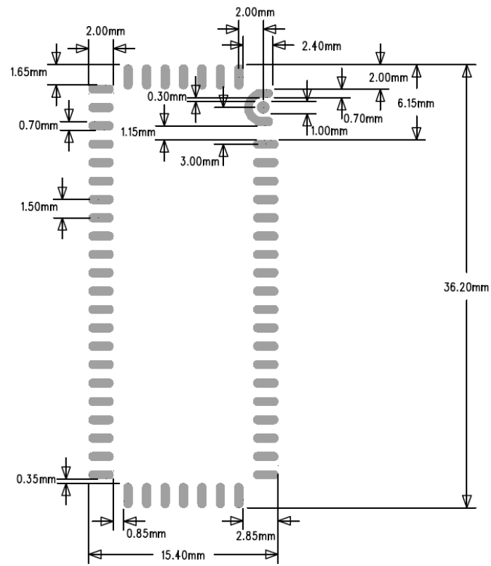
Figure 5: Recommended land pattern
