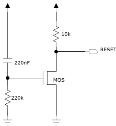
Figure 20: Example of a simple power on reset circuit.
