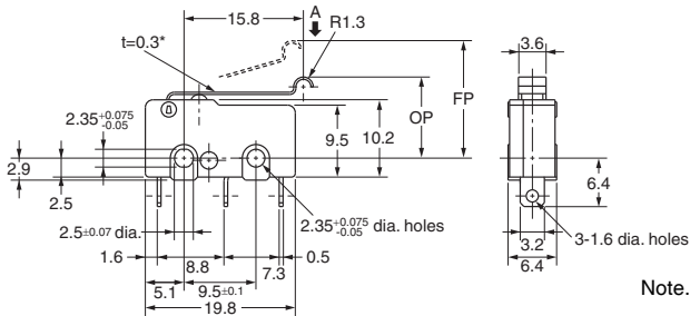
* Stainless-steel lever
