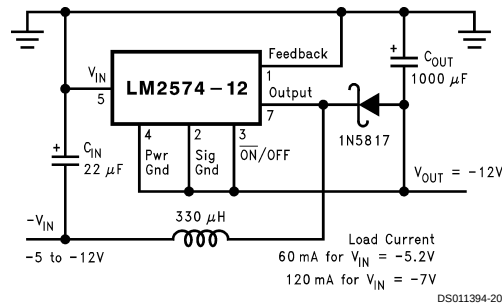
FIGURE 12. Negative Boost
