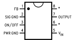
8-Lead DIP
