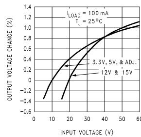
Line Regulation
