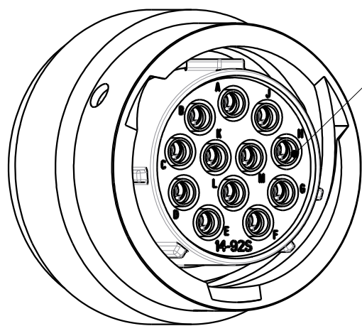
FEMALE CONNECTOR
