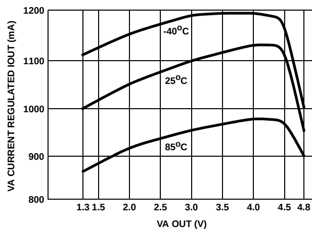
FIGURE 14. V_A CURRENT REGULATION vs. V_A OUT
