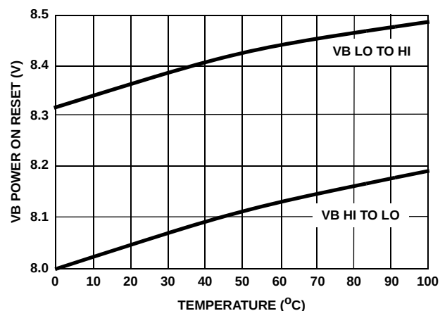
FIGURE 12. V_B POWER ON RESET VOLTAGE THRESHOLD
