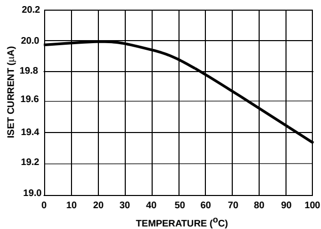
FIGURE 6. ISET SOURCE CURRENT
