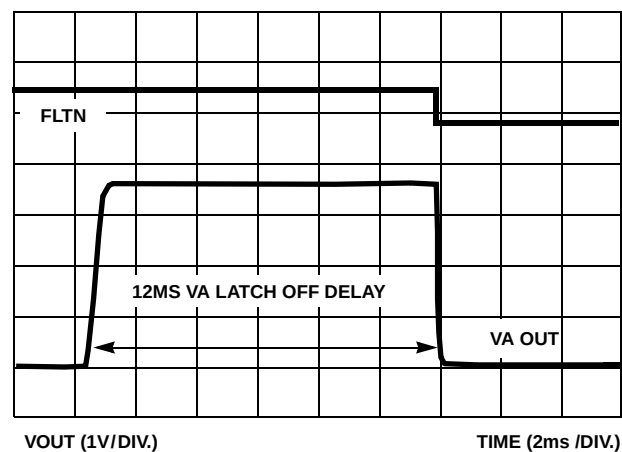
FIGURE 16. - V_A TURN-ON INTO 1.5A FAULT
