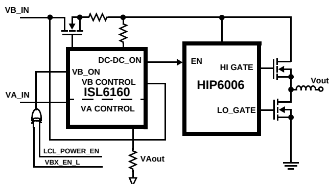
FIGURE 2. SIMPLIFIED ISL6160EVAL2 BLOCK DIAGRAM
