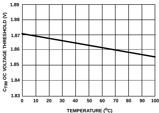
FIGURE 8. C_{TIM} OC VOLTAGE THRESHOLD
