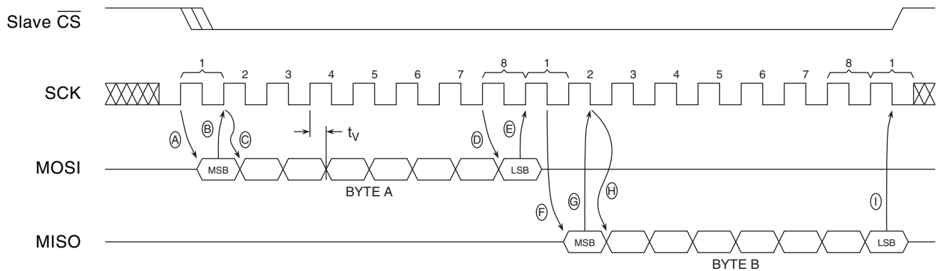
Figure 13-1. RapidS Operation
