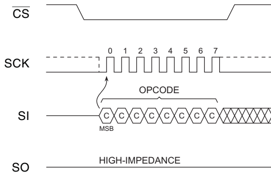
Figure 8-6. Chip Erase
