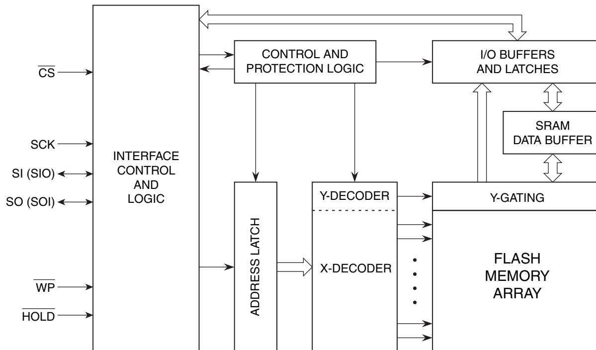
Figure 3-1. Block Diagram
