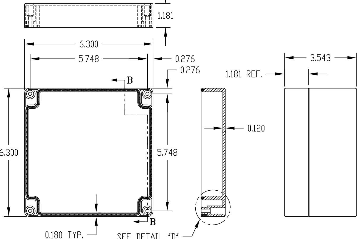
DETAIL "D"
