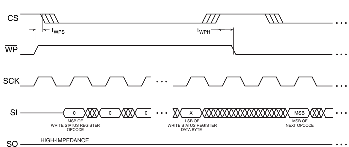
Figure 14-3. \overline{\text{WP}} Timing for Write Status Register Command When BPL = 1
