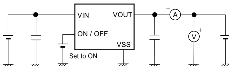
Figure 11 Test Circuit 3
