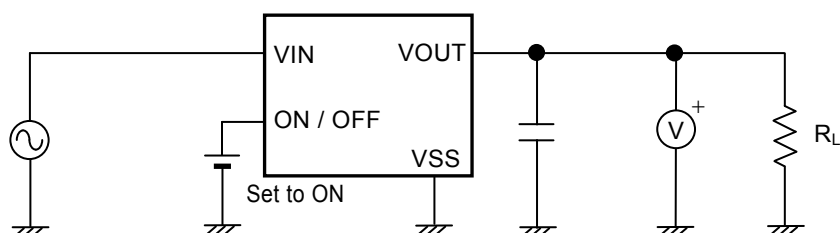
Figure 13 Test Circuit 5
