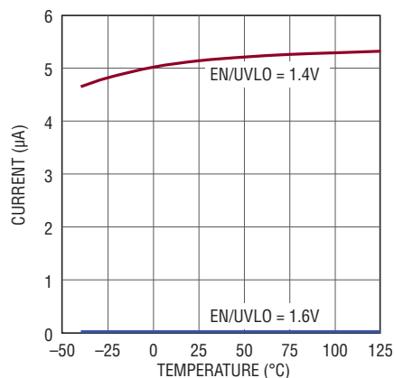
EN/UVLO Pin Bias Current
