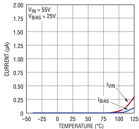
Shutdown Current
