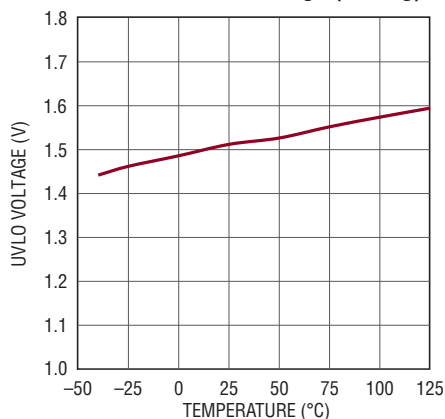
UVLO Threshold Voltage (Falling)
