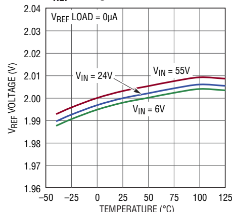
V_{REF} Voltage
