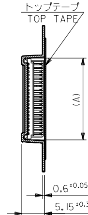
SECT. Z-Z
