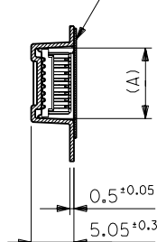
SECT. Z-Z
