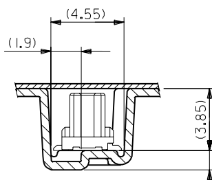
SECT. X-X (SCALE:5-1)
