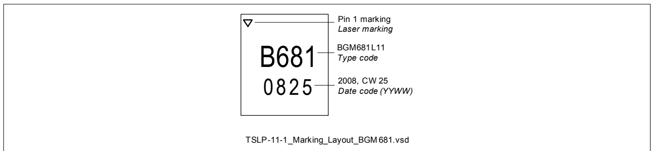
Figure 7 Marking Layout
