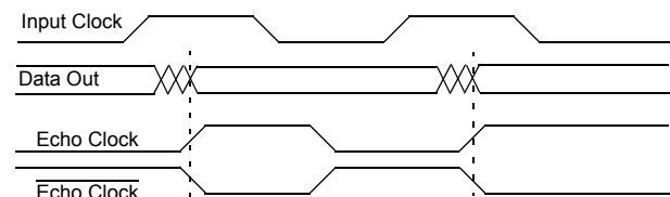
Figure 6. SDR Echo Clock Delay
