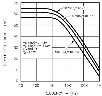
FIGURE 3. RIPPLE REJECTION VS. FREQUENCY
