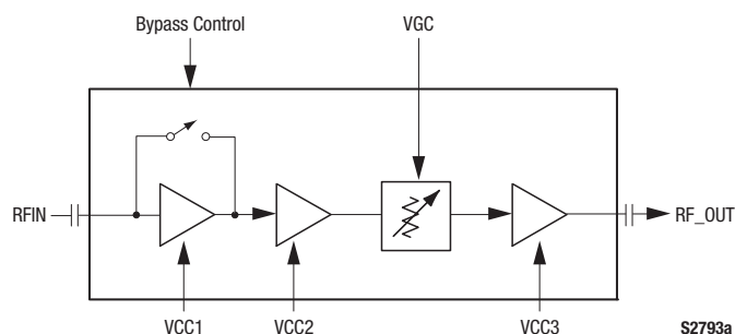
Figure 1. SKY65369-11 Block Diagram
