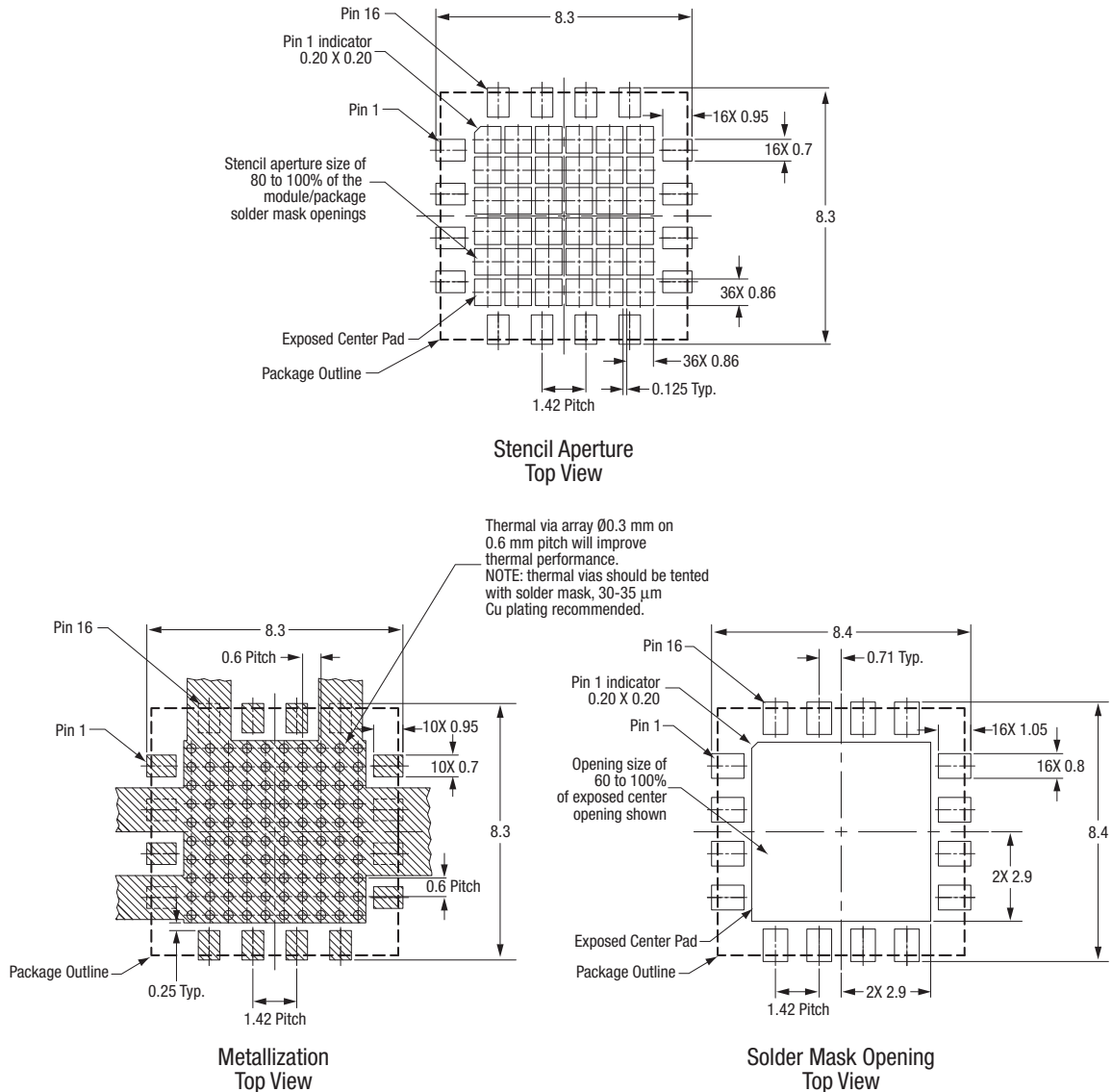
Figure 7. SKY65369-11 PCB Layout Footprint (Top View)
