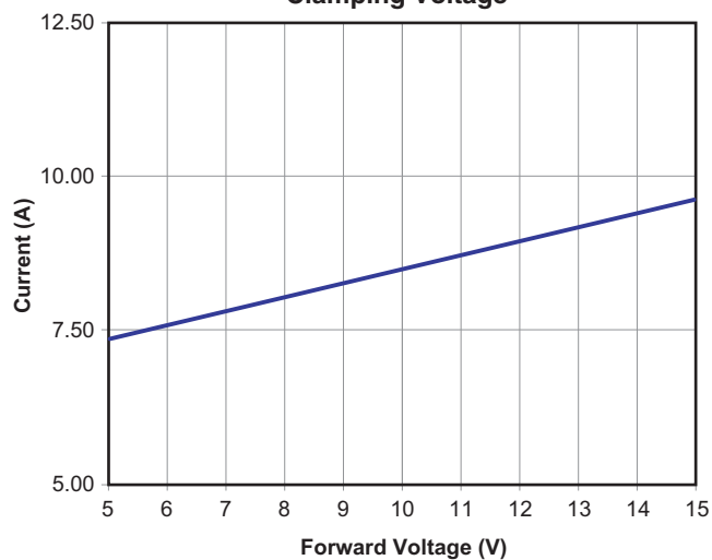
Clamping Voltage
