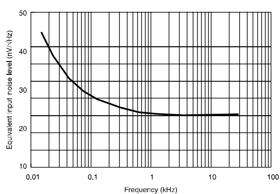
Figure 10: Equivalent input noise voltage vs. frequency
