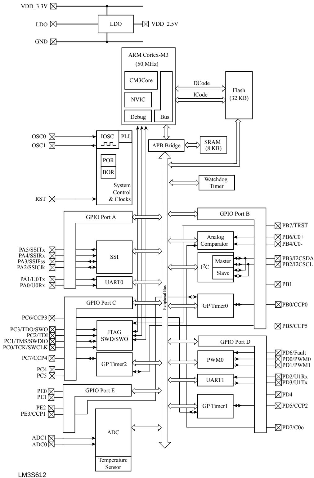
Figure 1-2. LM3S612 Controller System-Level Block Diagram
