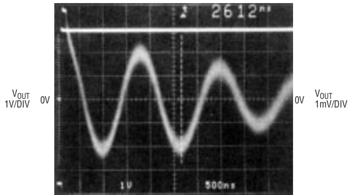
Settling Time Poor Bypass
