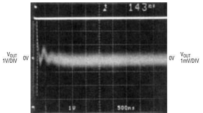
Settling Time Good Bypass
