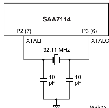
(1c) With fundamental quartz. Crystal load = 8 pF
