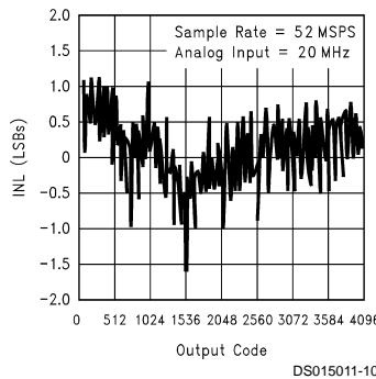
Integral Non-Linearity
