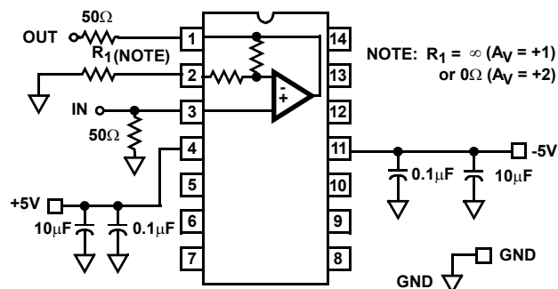
FIGURE 2. MODIFIED EVALUATION BOARD SCHEMATIC
