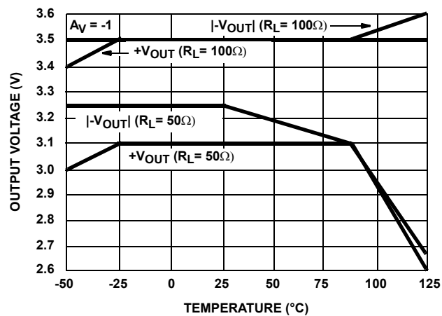
FIGURE 35. OUTPUT VOLTAGE vs TEMPERATURE
