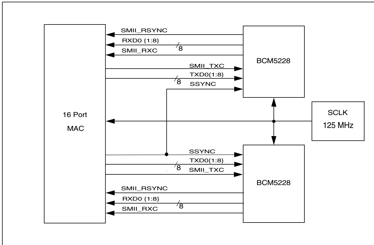
Figure 14: SMI Application using Source Synchronous Signals
