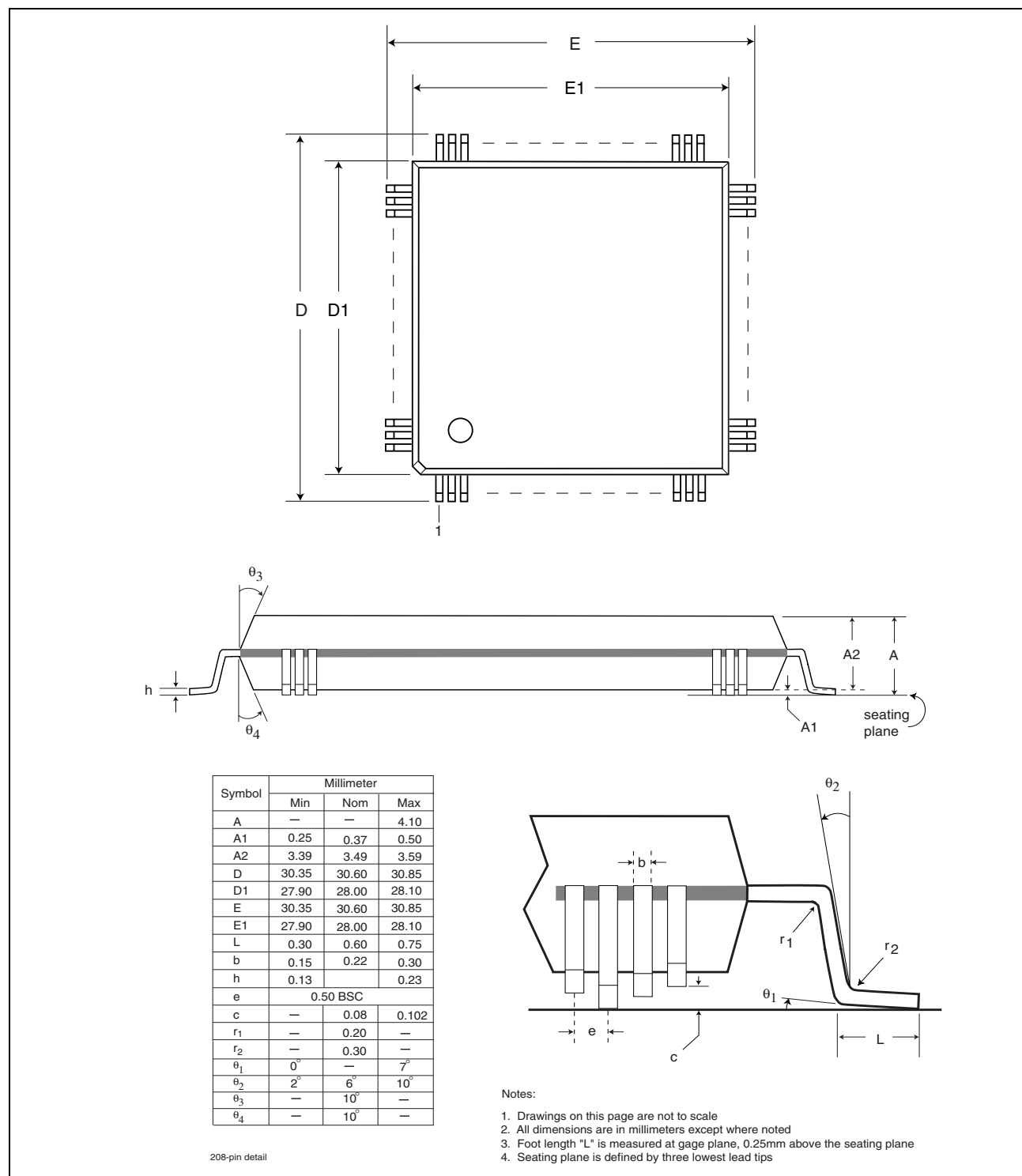
Figure 11: 208-Pin PQFP
