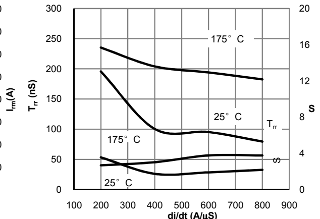
Fig 26: Diode Reverse Recovery Time and Softness Factor vs. di/dt ( V_{GE}=15V, V_{CE}=400V, I_F=15A )
