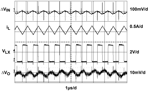
FIGURE 8. LOAD REGULATION @ V IN = 2.5V
