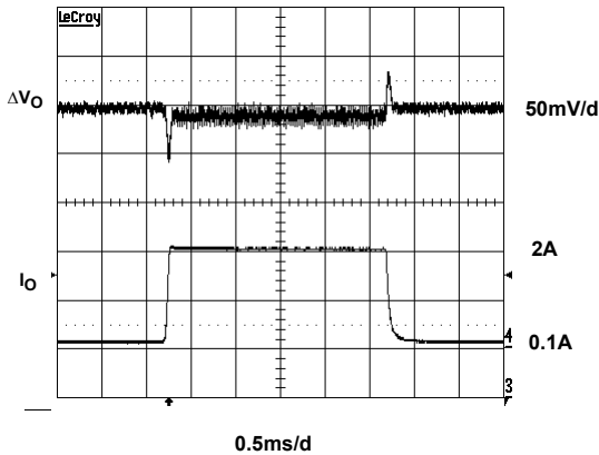
FIGURE 12. TRANSIENT RESPONSE
