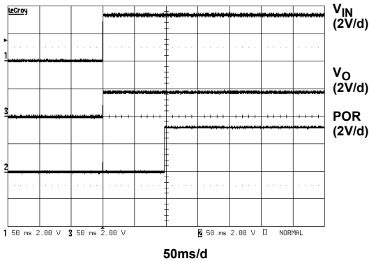
FIGURE 10. START-UP 2
