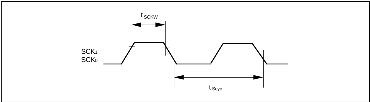
(2) SCI Input Clock Timing
