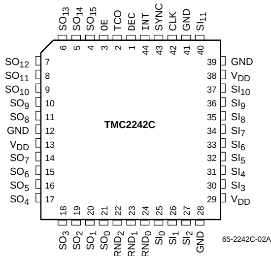
44 Lead PLCC
