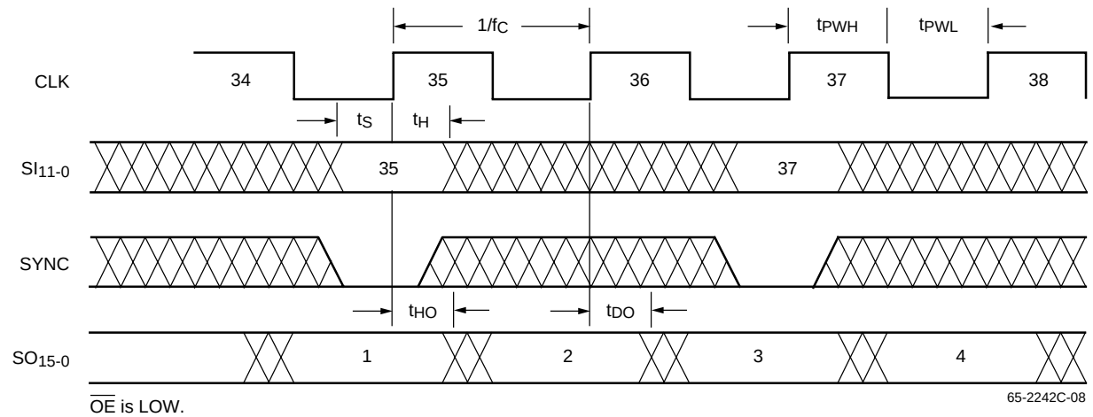
Figure 8. Interpolate Mode
