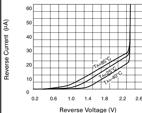
Reverse Characteristics
