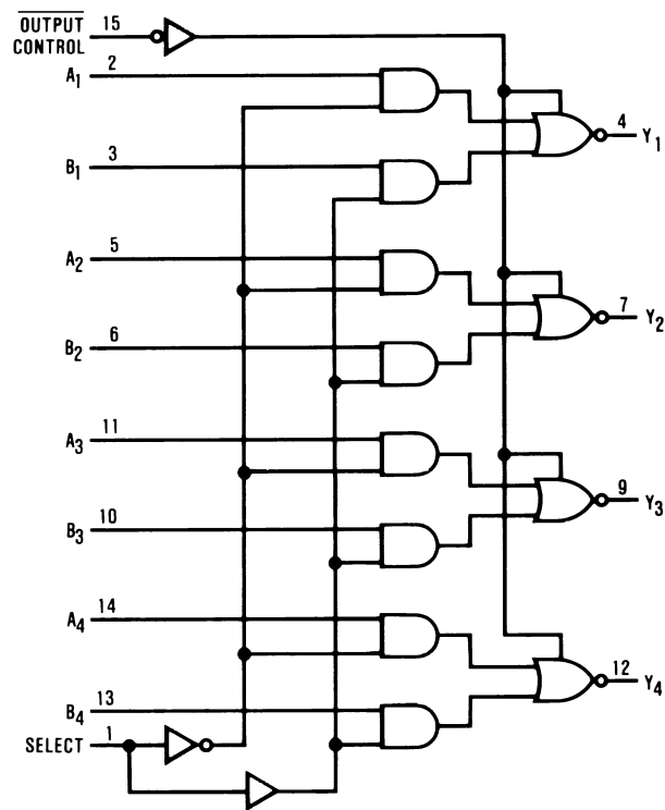
DM74AS258
