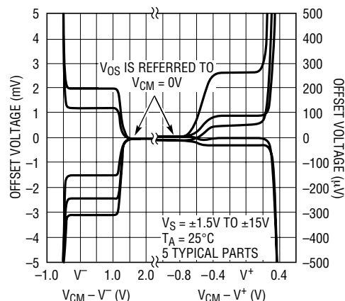
Offset Voltage Shift vs Common Mode
