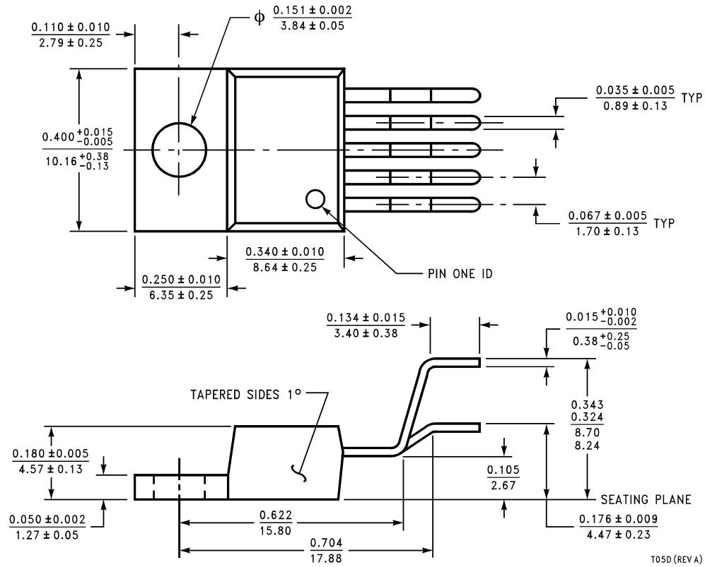
TO-220, Bent Staggered Leads (T)
