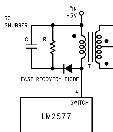
FIGURE 21. Snubber Circuit
