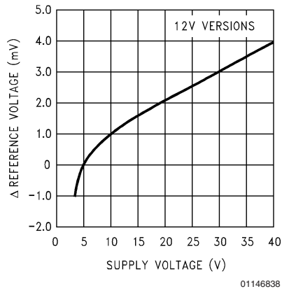
\Delta Reference Voltage vs Supply Voltage
